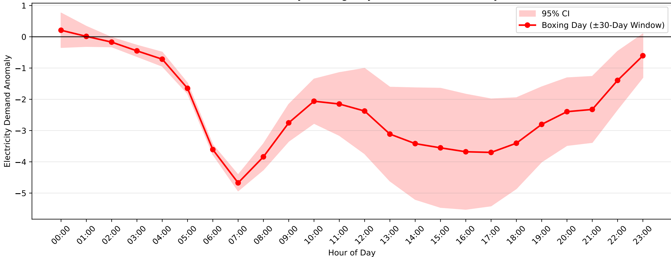
Mortdale Demand Anomaly: Boxing Day (2004–2017, \pm 30 -Day Window)
